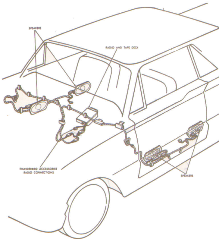
1966 THUNDERBIRD STEREO TAPE PLAYER
