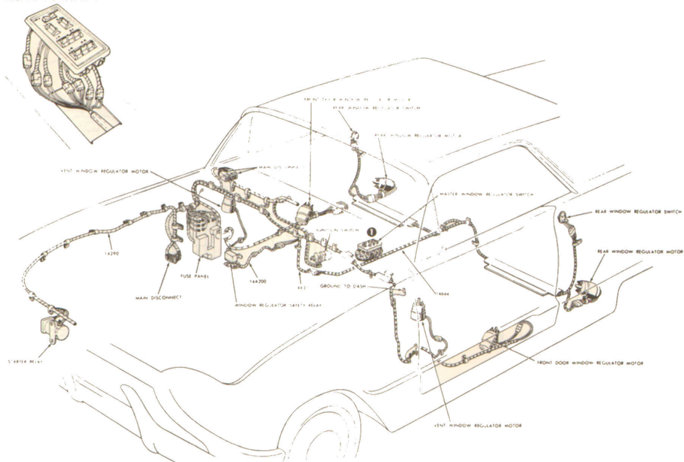
1966 THUNDERBIRD POWER WINDOWS
