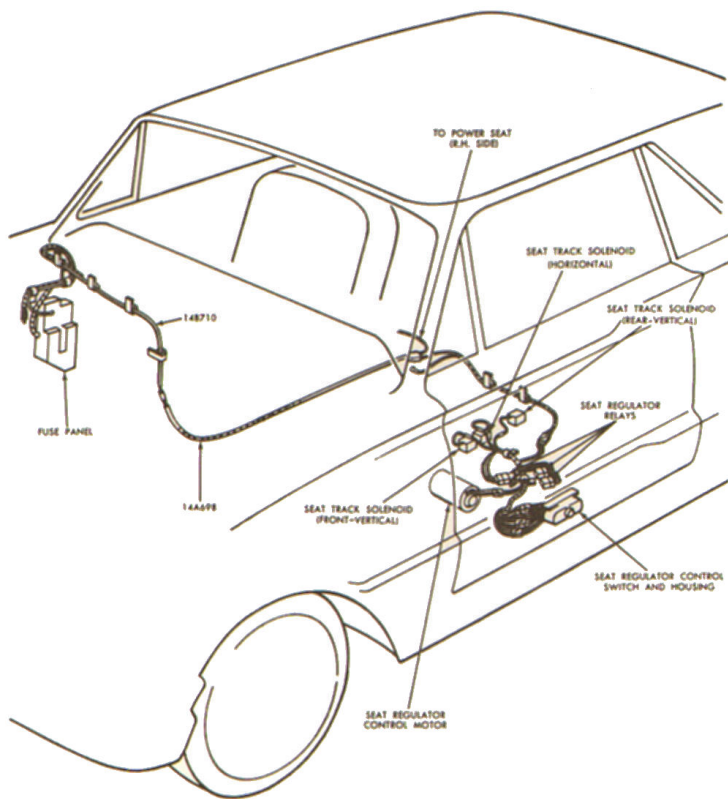
1966 THUNDERBIRD POWER SEAT (6-WAY)
