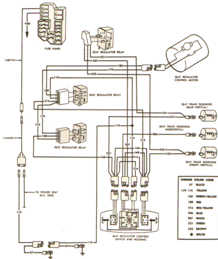
1966 THUNDERBIRD POWER SEAT (6-WAY)
