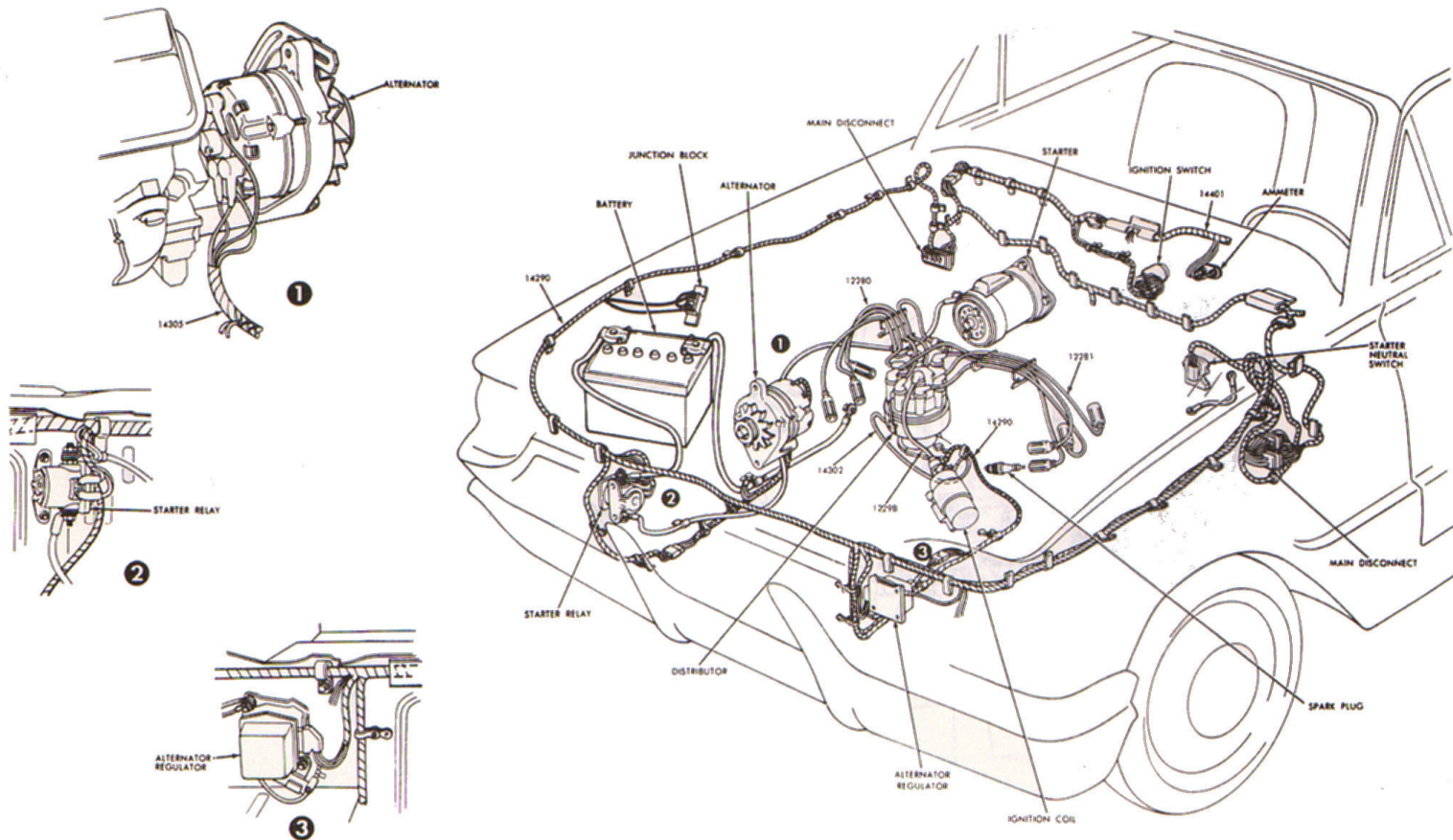
1966 THUNDERBIRD IGNITION, STARTING AND CHARGING
