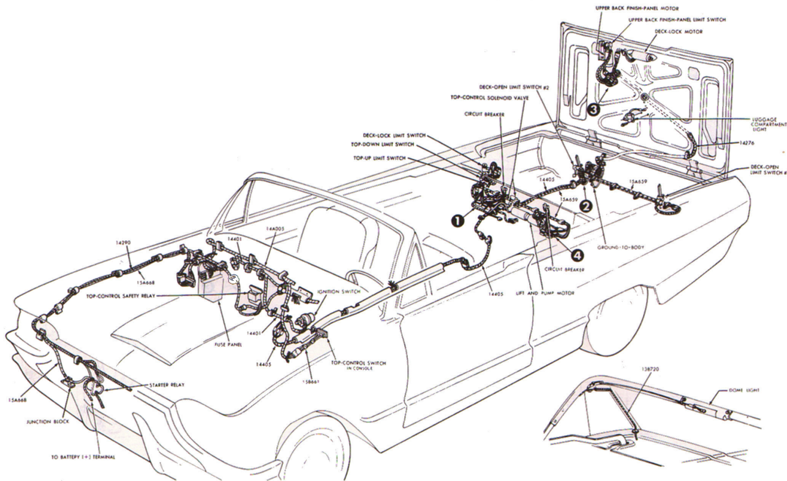
1966 THUNDERBIRD POWER TOP
