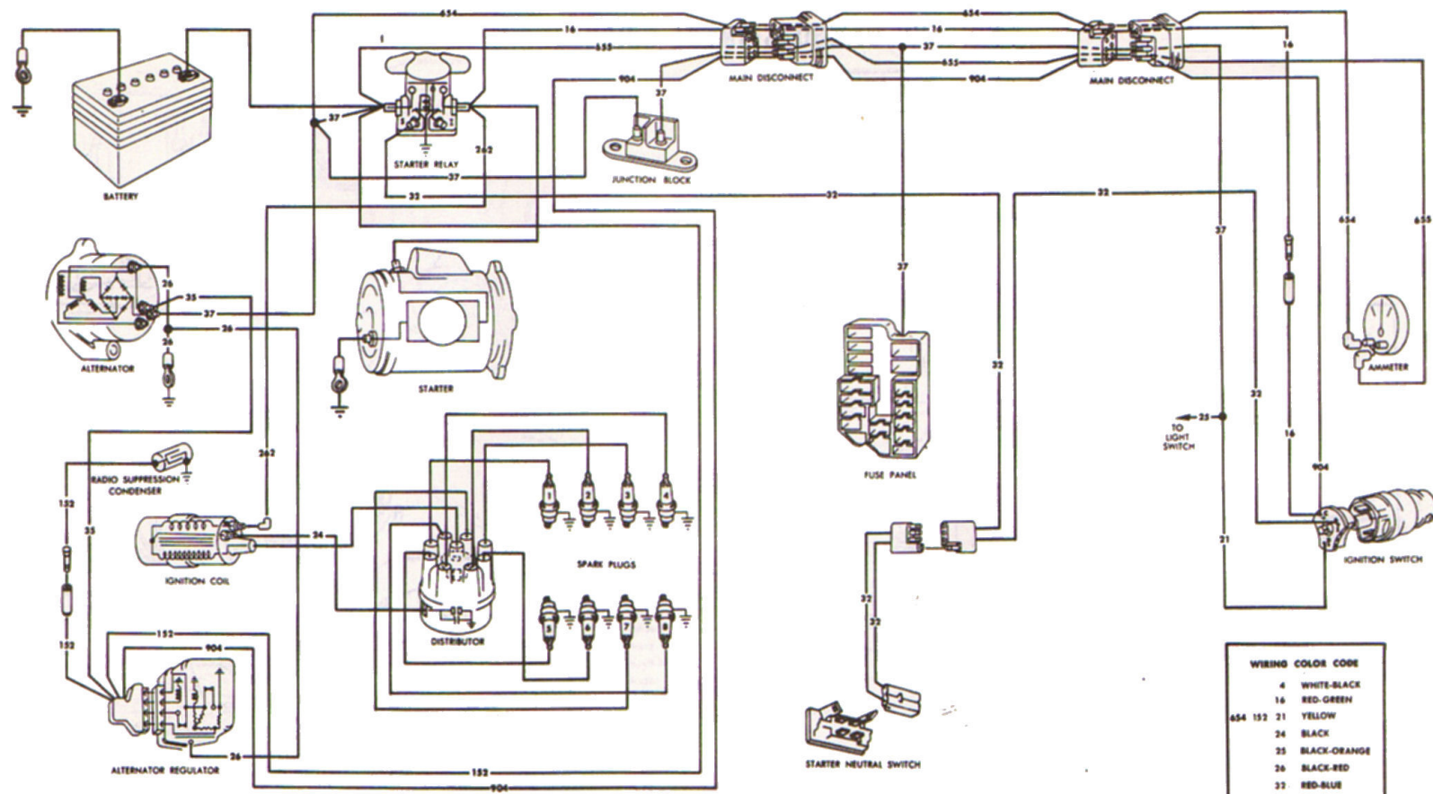
1966 THUNDERBIRD IGNITION, STARTING AND CHARGING
