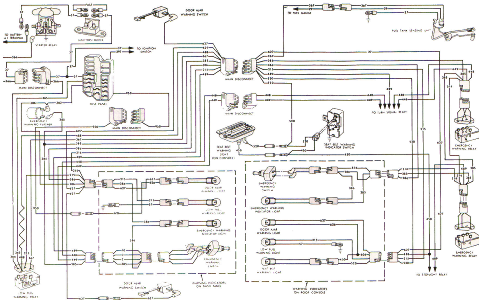
1966 THUNDERBIRD SAFETY CONVENIENCE PACKAGE
