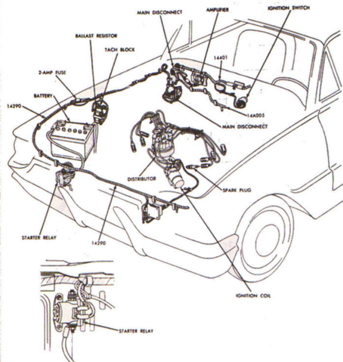
1966 THUNDERBIRD TRANSISTORIZED IGNITION
