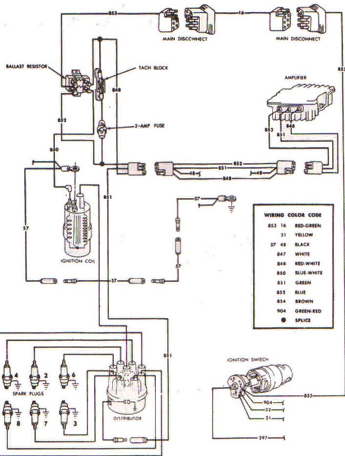
1966 THUNDERBIRD TRANSISTORIZED IGNITION
