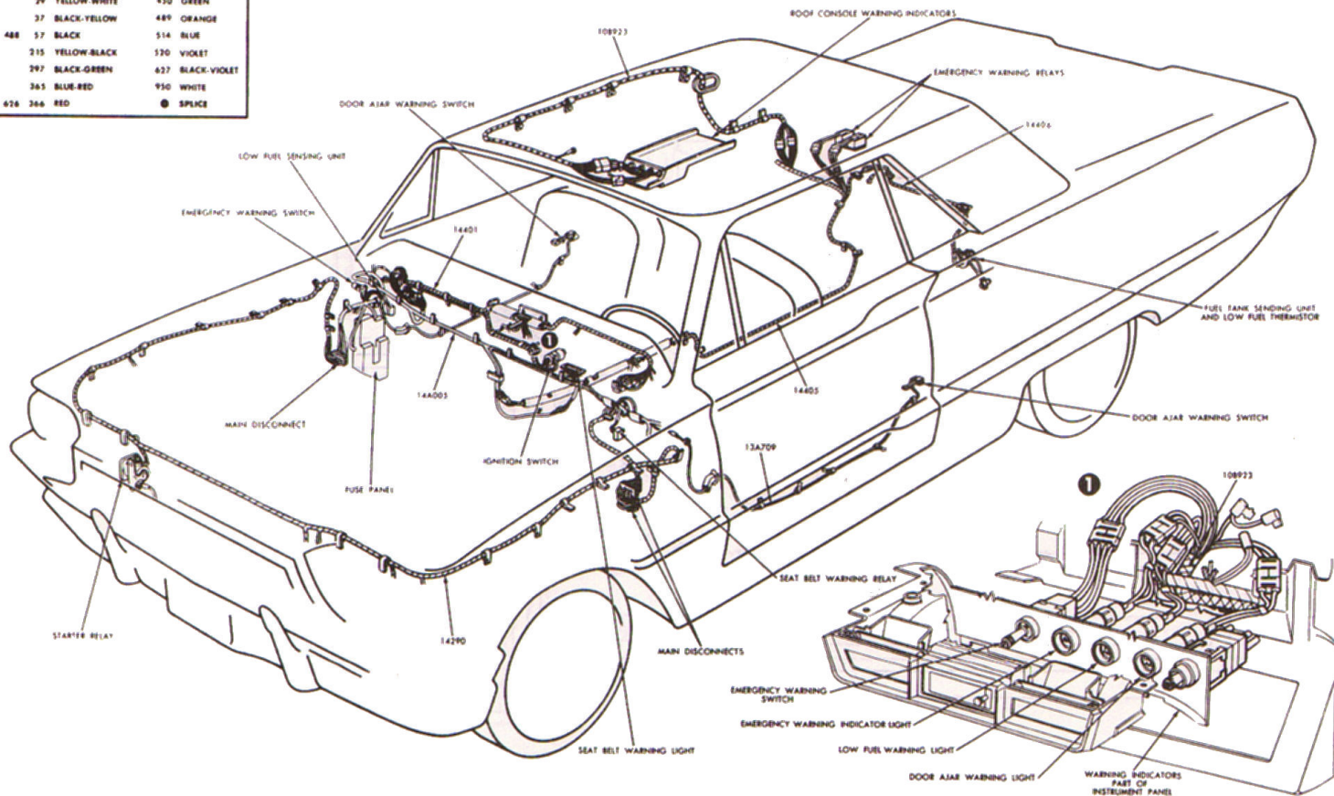
1966 THUNDERBIRD SAFETY CONVENIENCE PACKAGE
