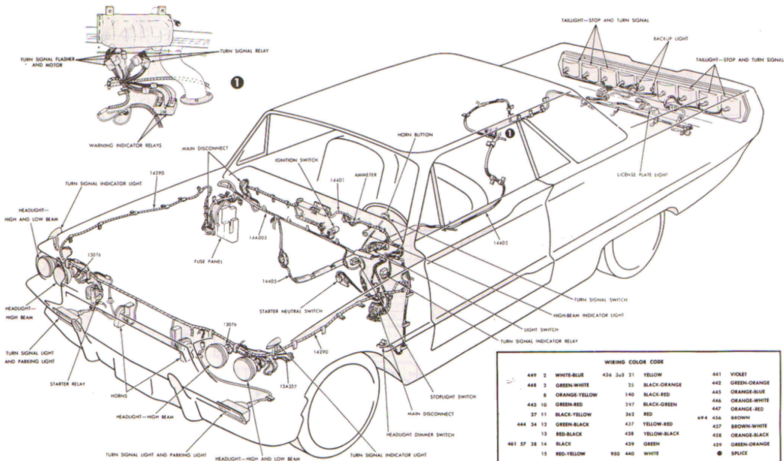
1966 THUNDERBIRD EXTERIOR LIGHTING
